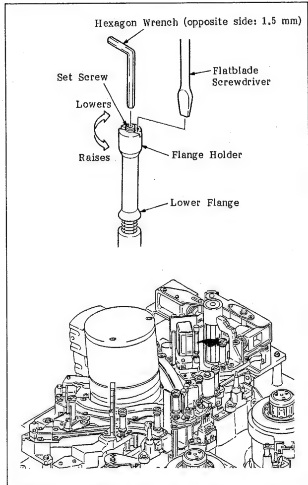
Fig. 9-5 Height Adjustment of the Guide Post
